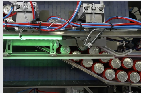
Bypass Mode Allows Loose Cans Through Without Facing
